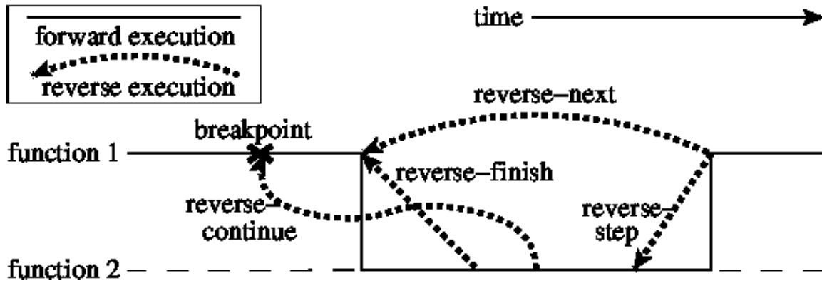
Figure 3: Reverse Commands.
